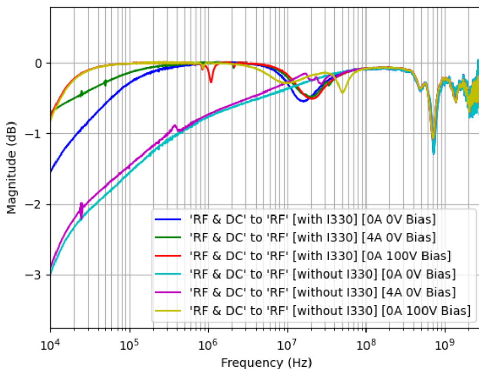
Insertion Loss 'RF & DC' to 'RF'
